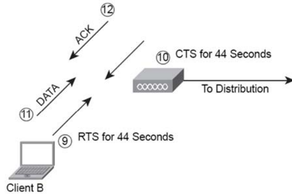
RTS/CTS
