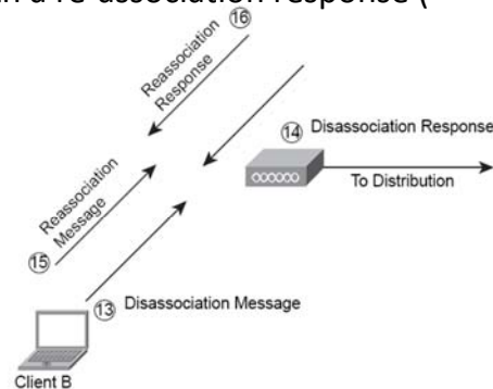
Reassociation
