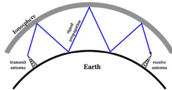
(b) Sky-wave propagation (2 to 30 MHz)
