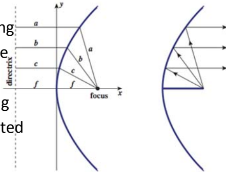
Dr. Ahmed ElShafee, ACU Spring 2016, Data Communication (a) Parabola (b) Cross-section of parabolic antenna showing reflective property
