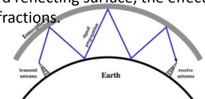
(b) Sky-wave propagation (2 to 30 MHz)
