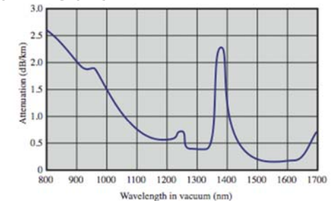
(c) Optical fiber (based on [FREE02])
