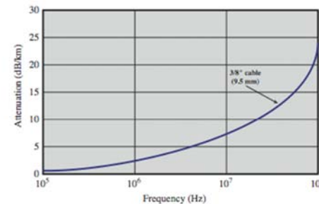
(b) Coaxial cable (based on [BELL90])
