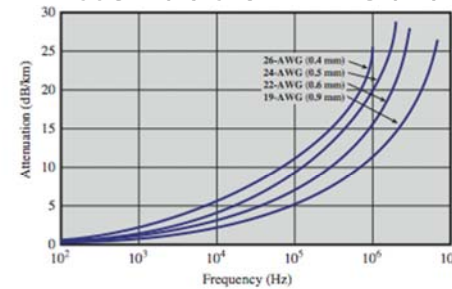
(a) Twisted pair (based on [REEV95])
