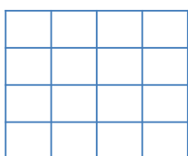
CipherState
