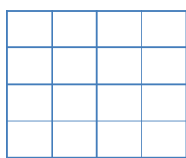
CipherState
