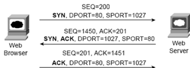
TCP Connection Establishment
