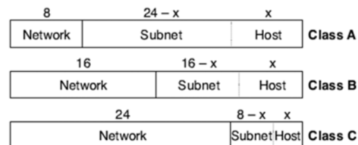
Address Formats When Subnetting Is Used
