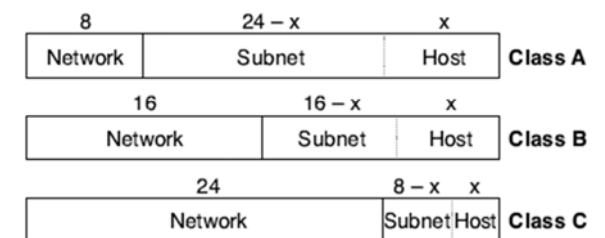
Address Formats When Subnetting Is Used
