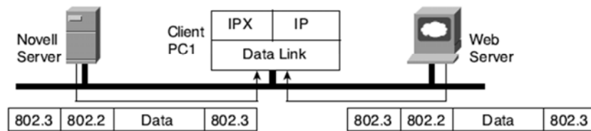
Multiplexing Using Data-Link Type and Protocol Fields
