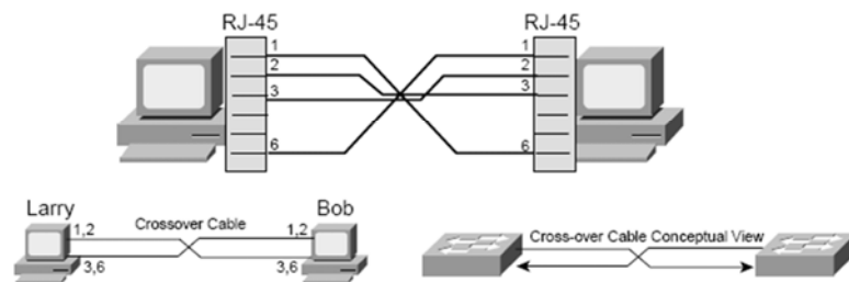
Crossover Ethernet Cable
