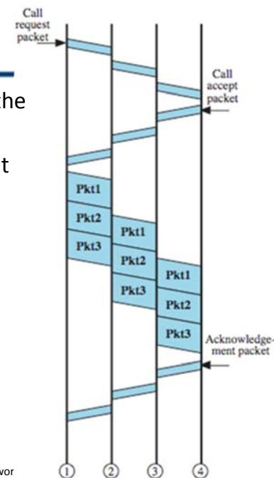
(b) Virtual circuit packet switching
