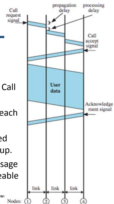
(a) Circuit switching
